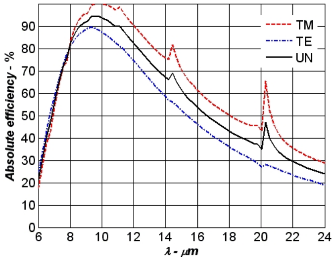
Type R11-001
